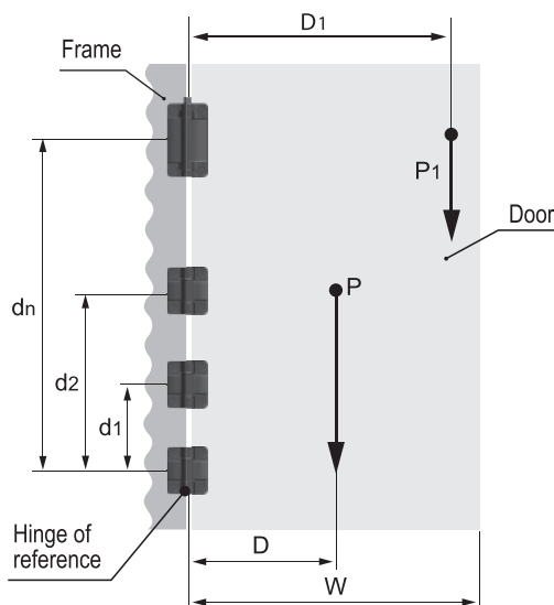
Hinged door on a vertical axis
