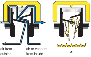
Operating layout
