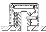
Assembly with grub screw and ball with adjustable pressure spring
