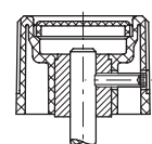
Assembly with grub screw
