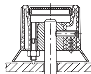
Assembly with grub screw and bolt plunger with locking nut
