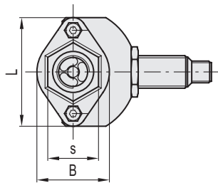
HVF-E (G3/8 - G1/2)
