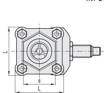
HVF-E (G3/4 - G1)
