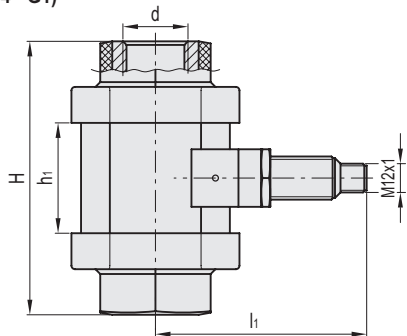
HVF-E (G3/4 - G1)
