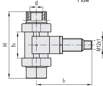
HVF-E (G3/8 - G1/2)
