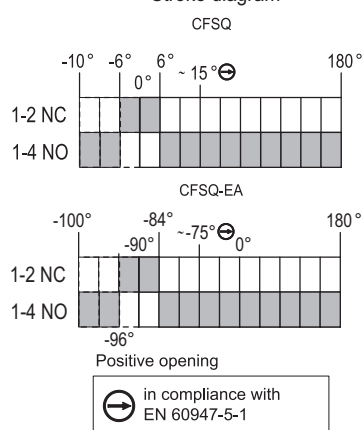
Stroke diagram
