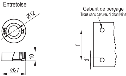
HCK-E-ST-KN HCK-E-STL-KN
