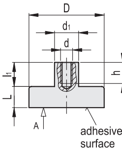
RMC-HF RMC-HF-SST
