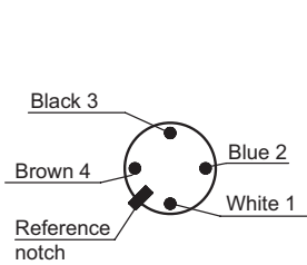
Wiring connector version
